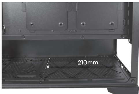
PSU Length
